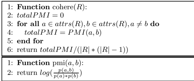
Figure 8: The coherency score measures how well attributes of a schema fit together. Probabilities for individual attributes are derived using statistics in the ACSDB.
